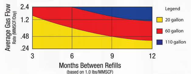
610 Storage Tank Selection Chart
